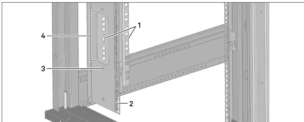
Figure 4.6 EIA-rail Features
