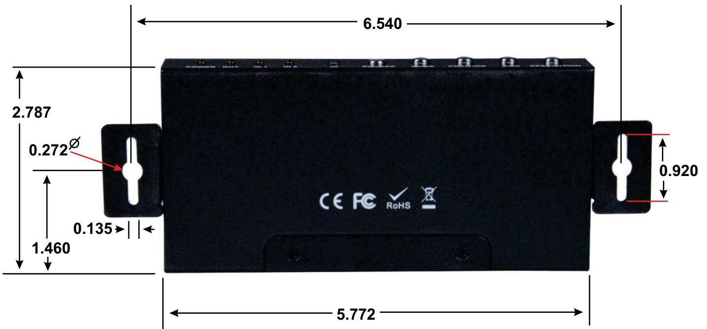
Bottom View
