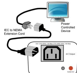
Fig. 2 Connect Device
