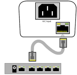
Fig. 1 Connect Network
