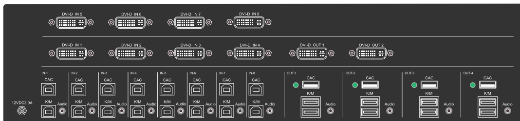
Figure 5-4: SDVN-82-X Rear panel
