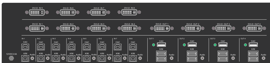
Figure 5-6: SDVN-84-X Rear panel
