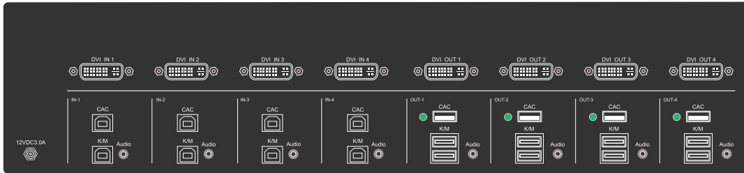
Figure 5-2: SDVN-44-X Rear panel
