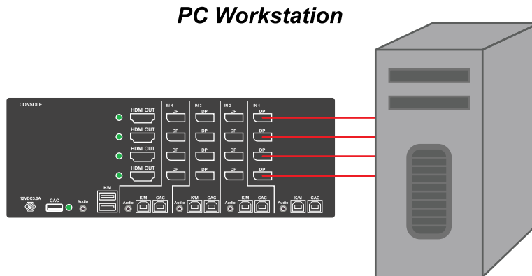
Figure 7-1: SDPN-4Q-P
