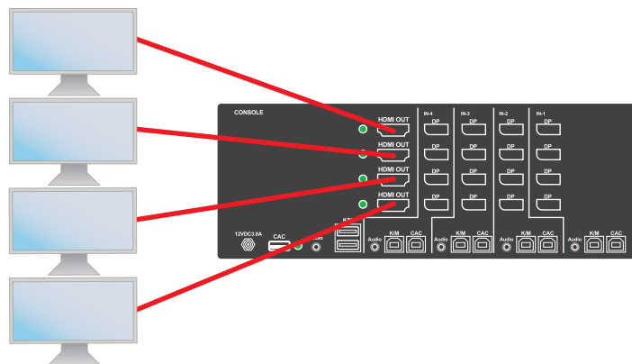
Figure 7-2: SDPN-4Q-P
