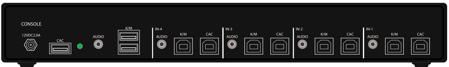
Figure 4-2: SA-KMN-4S-P Rear panel
