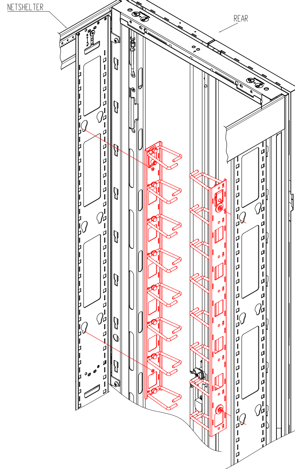
TYPICAL TOOLLESS MOUNTING
