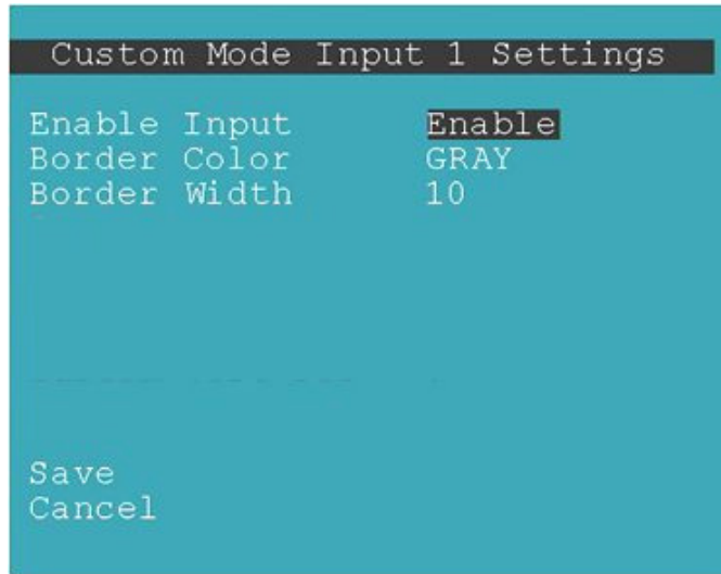
Figure 64- OSD- Custom Screen Mode Settings
