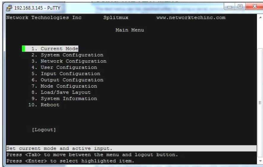
Figure 28- Text Menu-Main Menu
