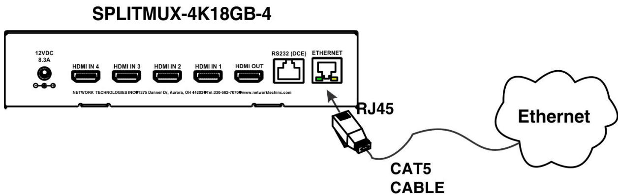
Figure 6- Ethernet connection
