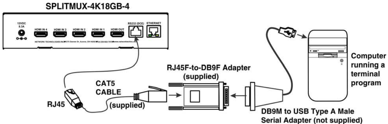
Figure 5- RS232 Terminal Connection
