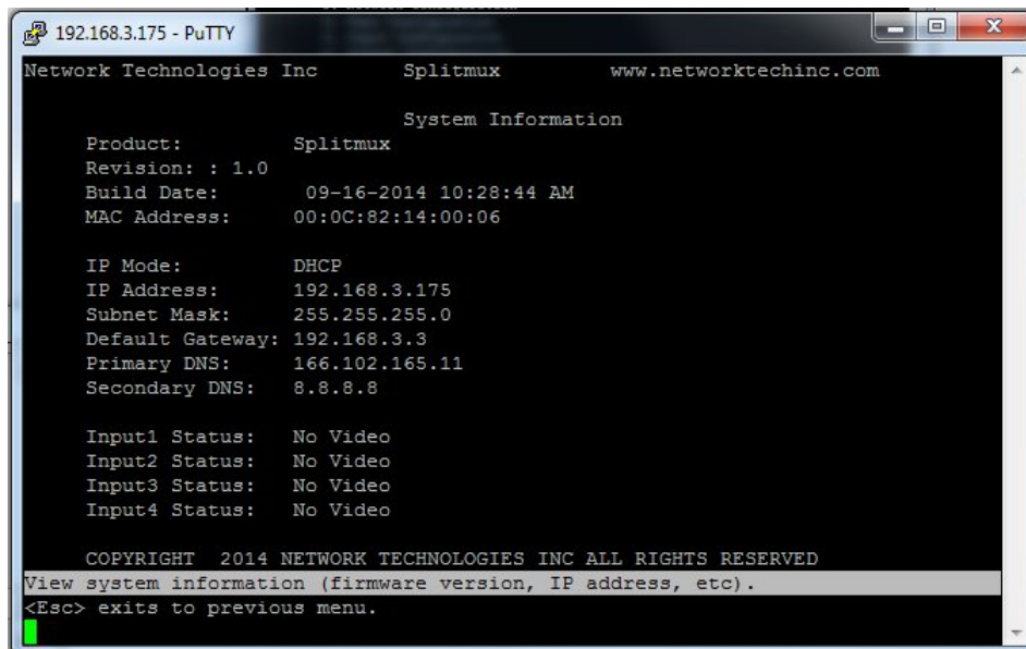
Figure 51- Text Menu- System Information
