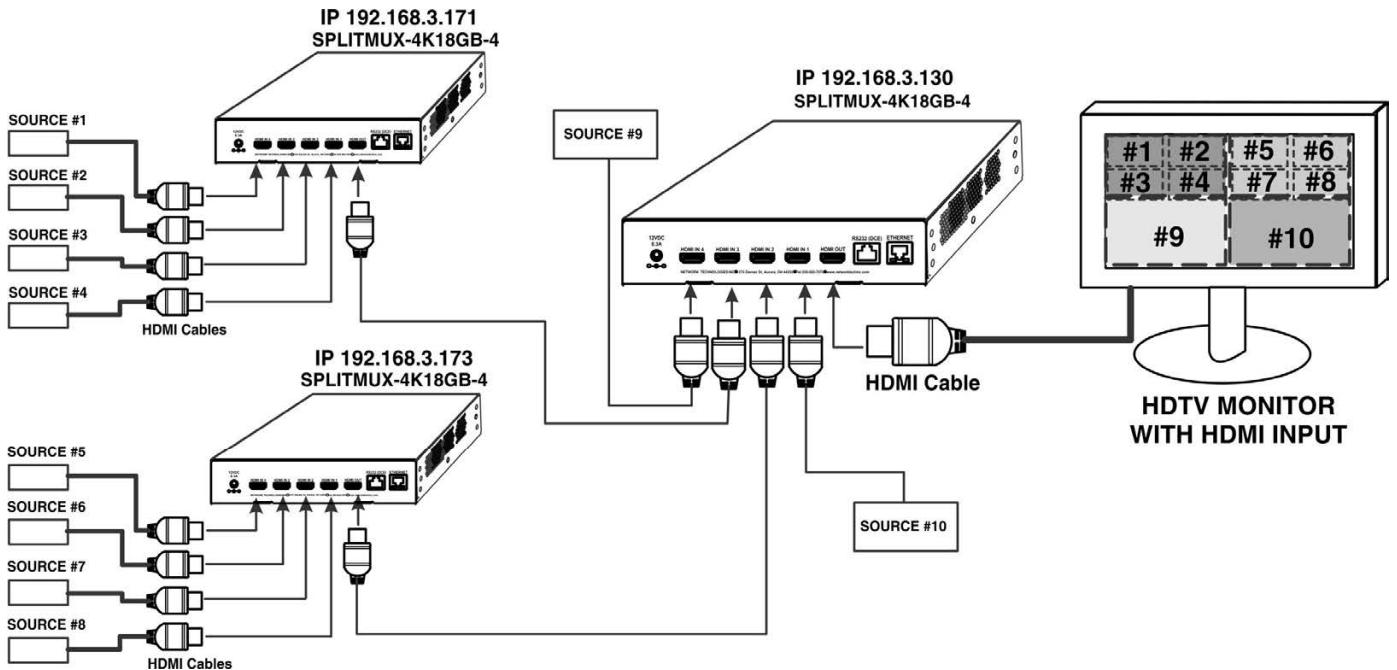
Figure 22- Cascading SPLITMUXs
