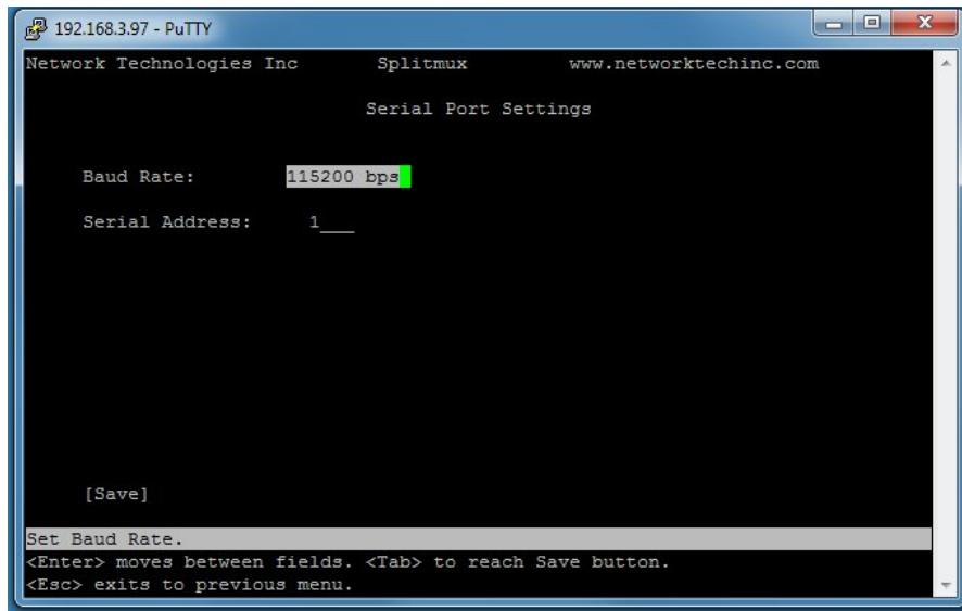
Figure 32- Text Menu- Serial Port Settings
