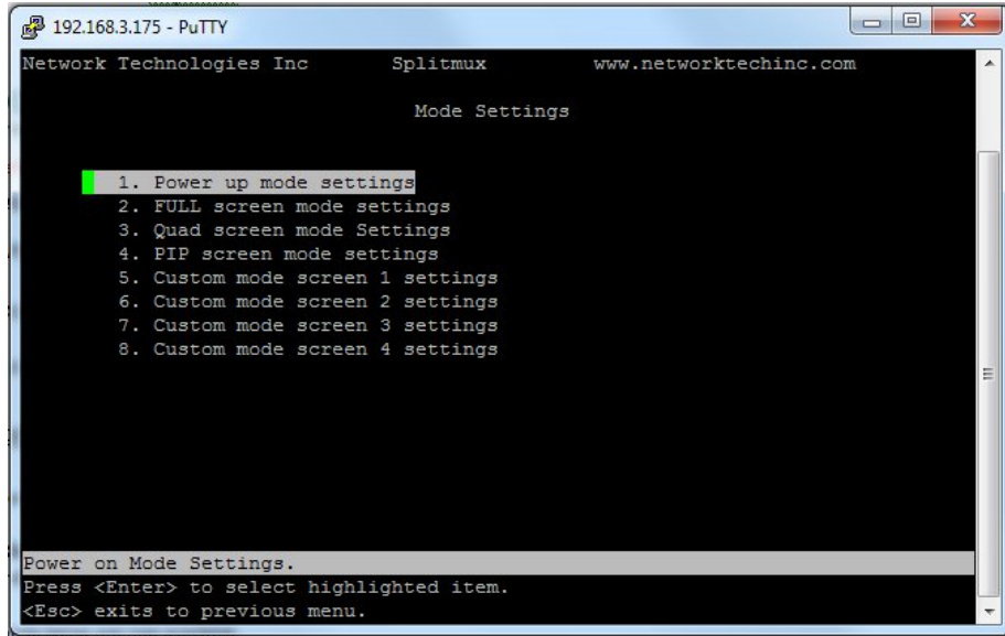
Figure 44- Text Menu- Mode Settings Menu
