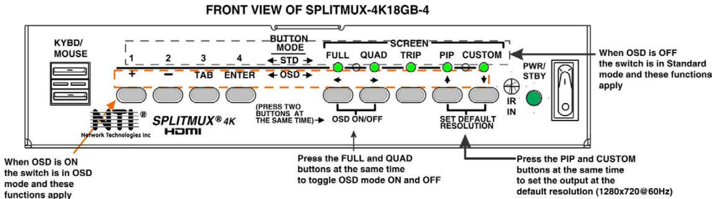
Figure 8- Front Panel Button Functions
