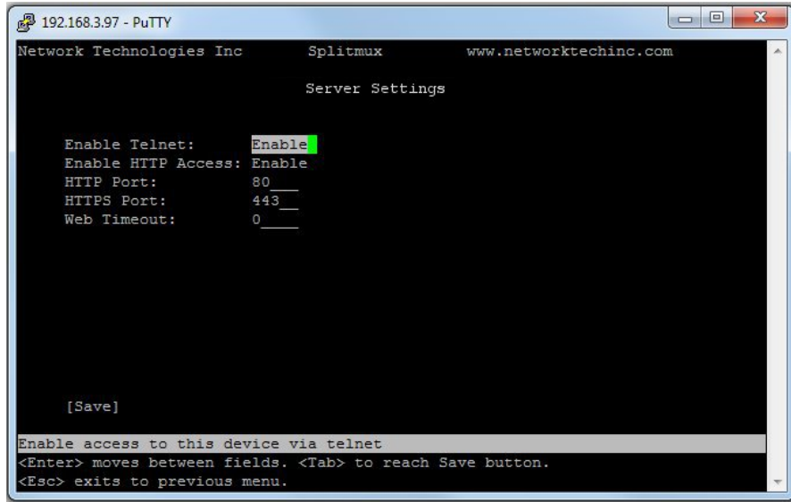
Figure 37- Text Menu-Server Settings
