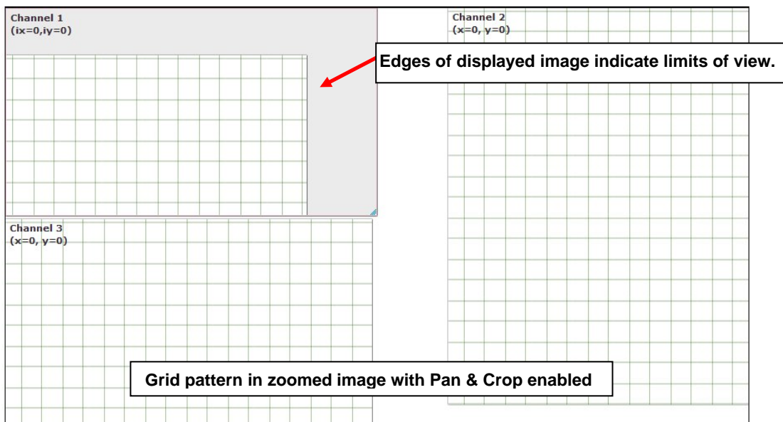
Figure 21- Pan and Crop Enabled
