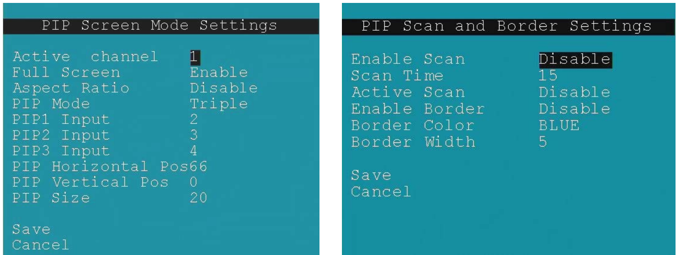
Figure 63- PIP Screen Mode settings
