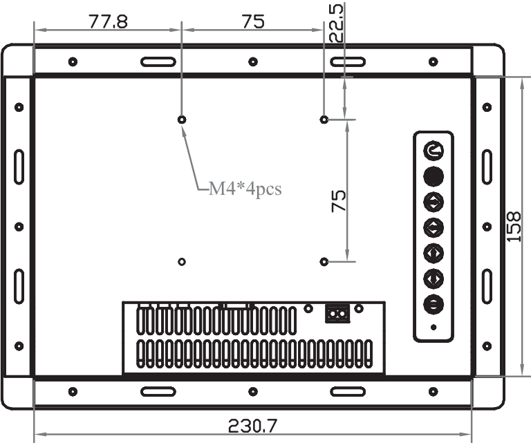
Rear View
