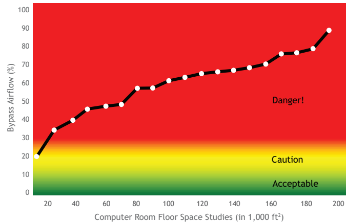
Bypass Airflow in Nineteen Computer Rooms Totaling 204,400 ft 2
