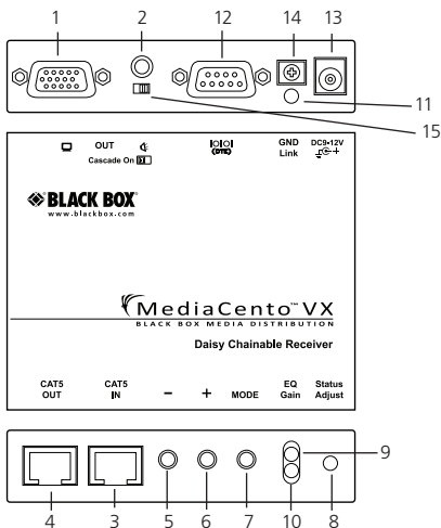
Figure 2-5. AVX-VGA-TP-CSRX front and back panels.
