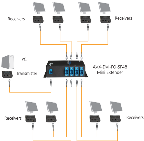
Figure 2-10. AVX-DVI-FO-SP8.
