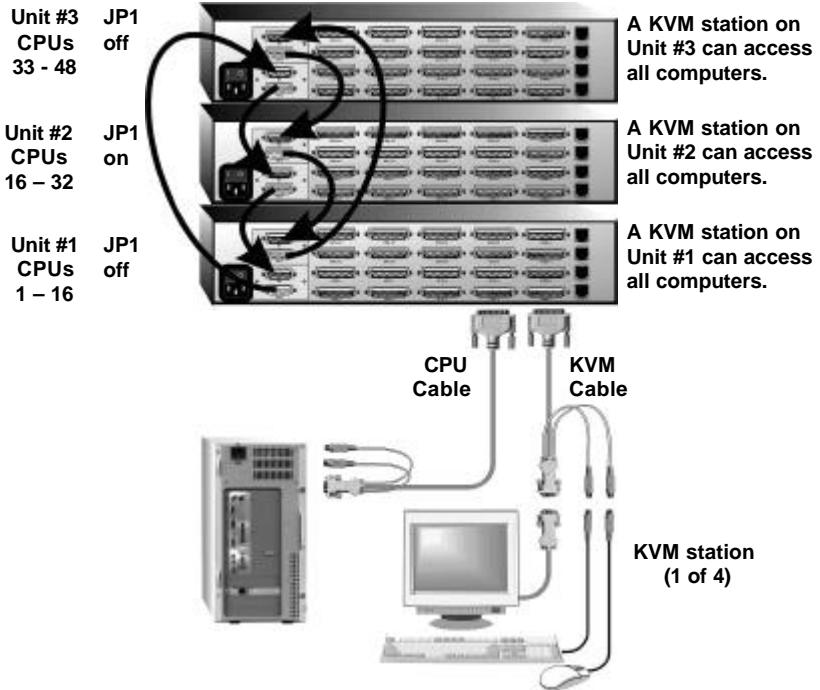
Figure 5. Ring configuration
