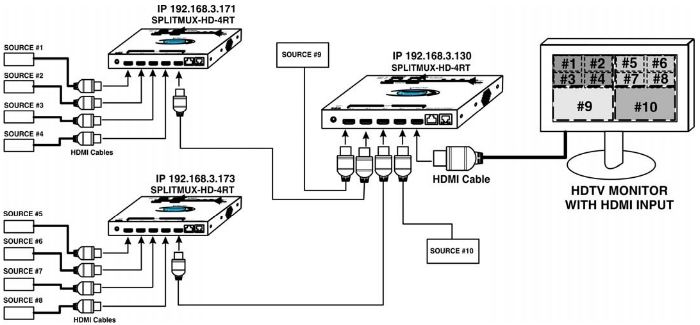
Figure 31- Cascading SPLITMUXs
