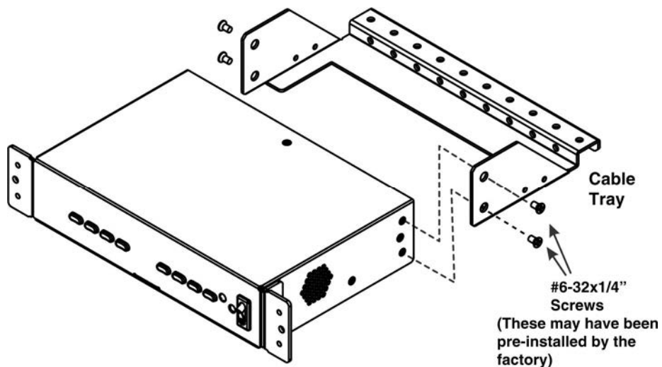
Figure 2- Attach cable tray (if applicable)
