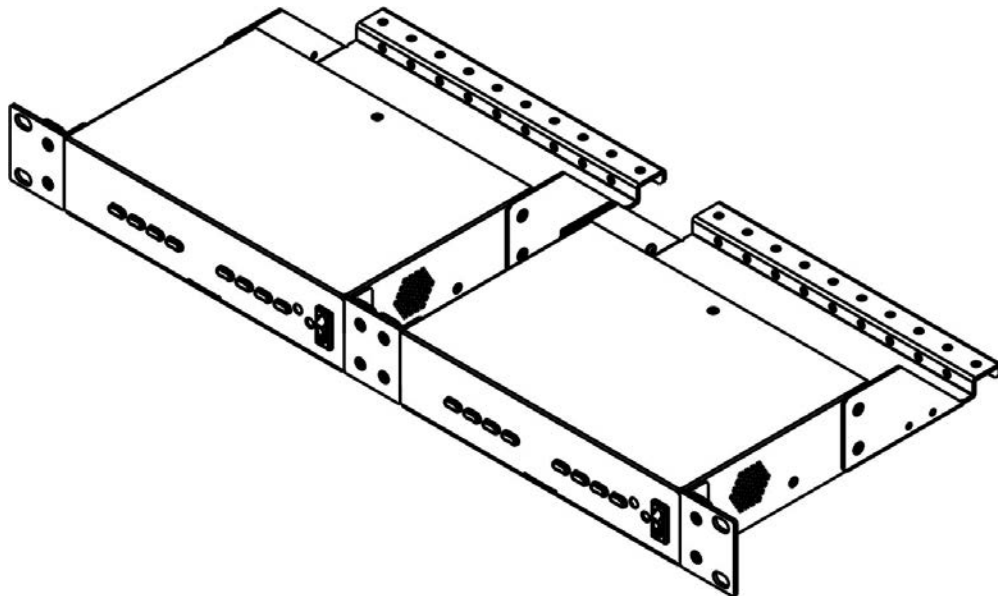
Figure 8- Assembled SPLITMUX-HD-4RT-2R
